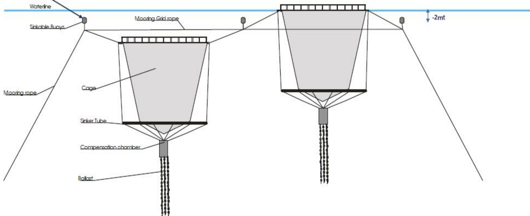
Schematic Description of the sinkable buoys layout
